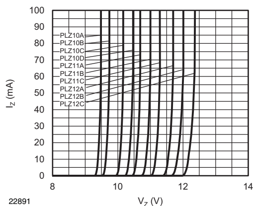
Fig. 6 - Breakdown Characteristics
