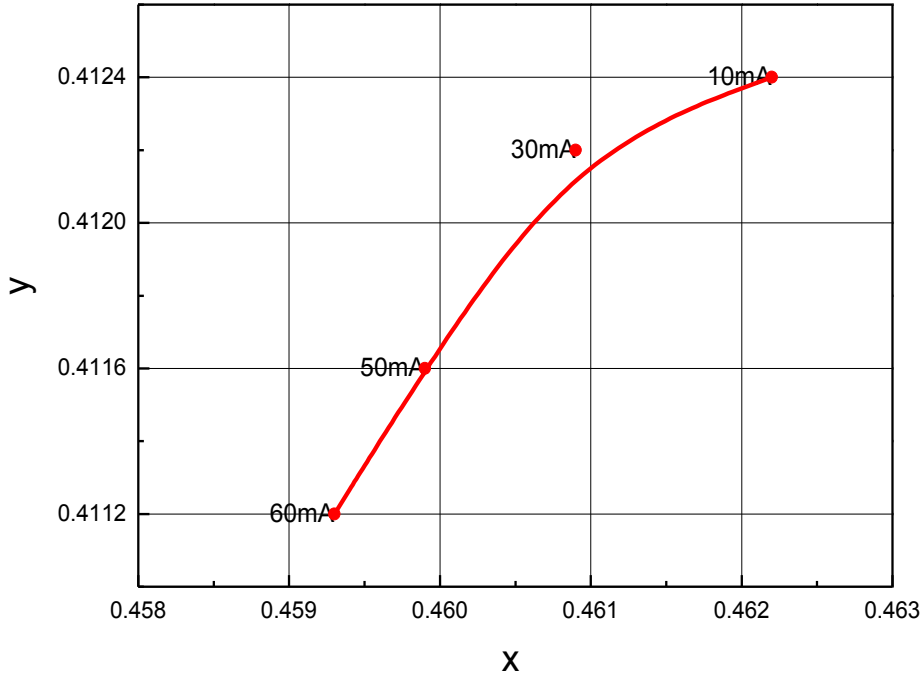
Fig 5. Forward Current vs. CIE X,Y Shift, T_j = 25^\circ\text{C} (2600-4200K)
