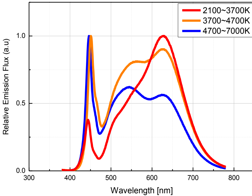
Fig 1. Color Spectrum, T_j = 25^\circ\text{C} , I_F = 50\text{mA}
