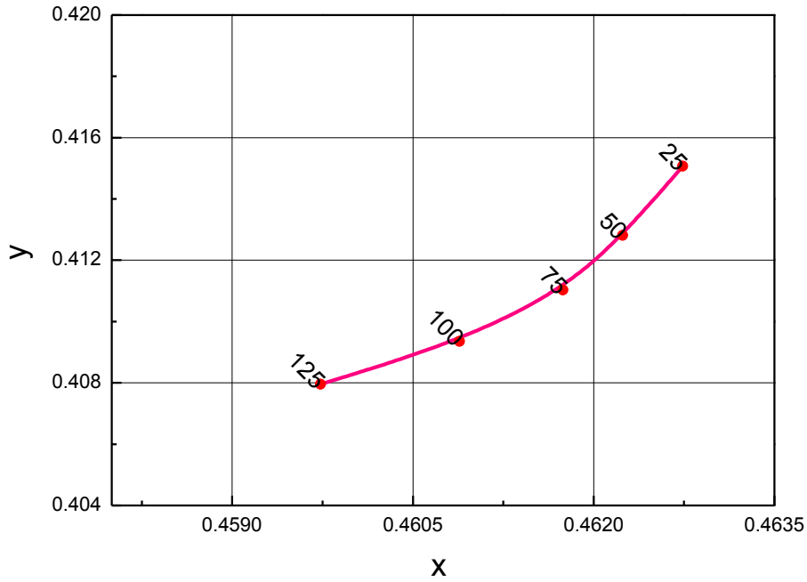
Fig 8. Chromaticity Coordinate vs. Junction Temperature, I_F=50\text{mA} (2600-4200K)
