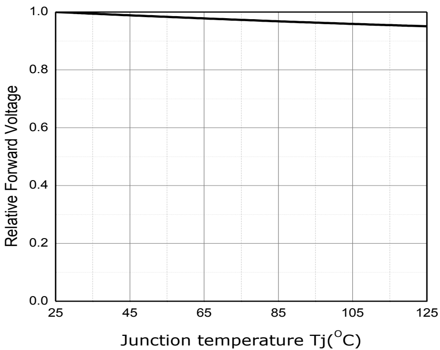
Fig 7. Junction Temperature vs. Relative Forward Voltage, I_F=50\text{mA}
