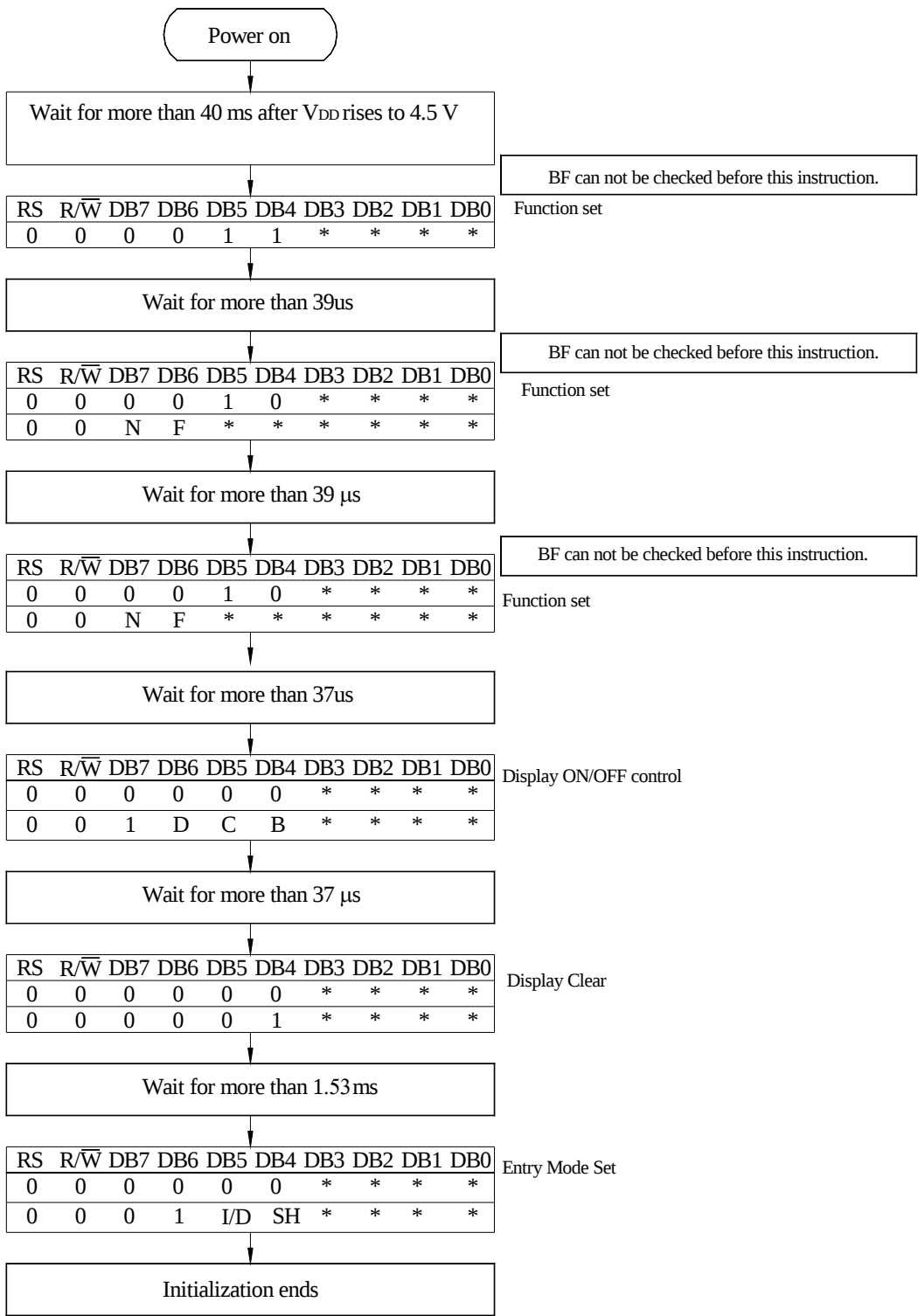
4-Bit Ineterface
