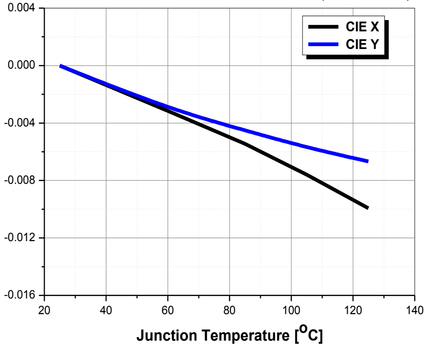
Fig 8. Junction Temp. vs. CIE X, Y Shift, I_F=60mA (CRI80)
