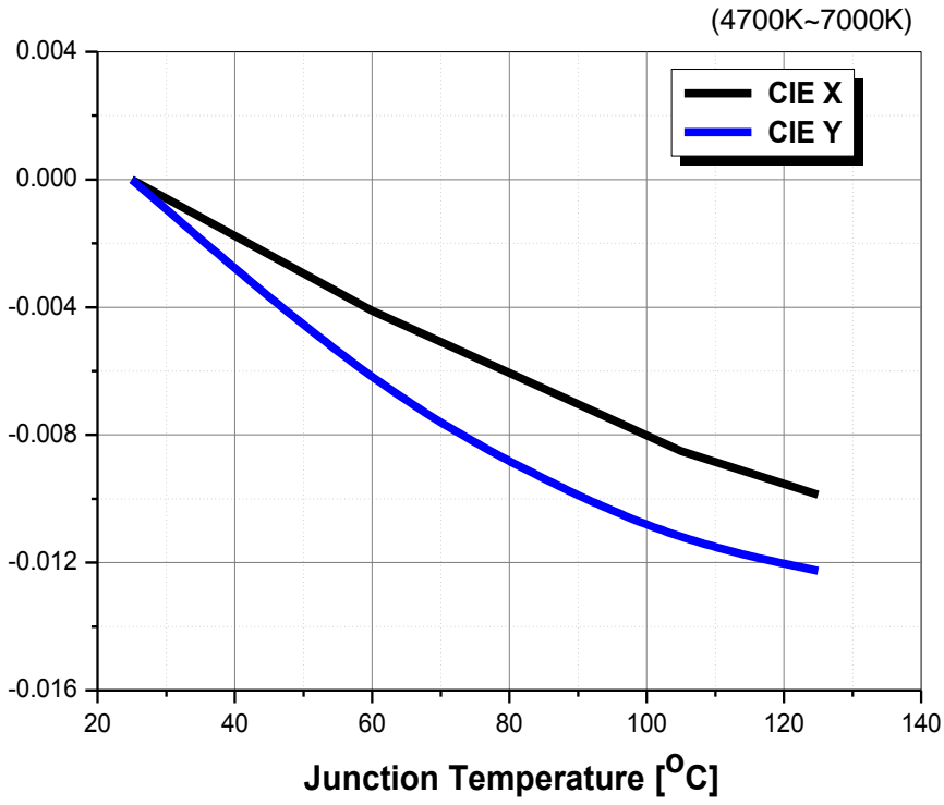
Fig 8. Junction Temp. vs. CIE X, Y Shift, I_F=60mA (CRI80)
